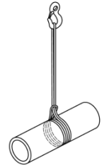
Figure C.1 - Élingage bagué double
