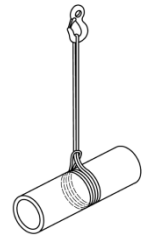
Figure C.1 – Élingage bagué double
